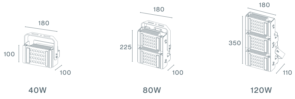
DIMENSIONS (mm)
