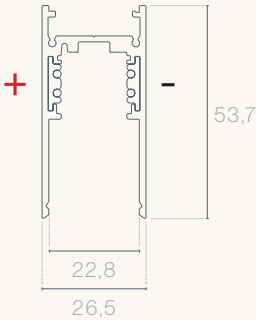
Dimensions (mm)
