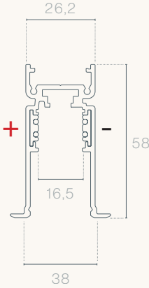
Dimensions (mm)
