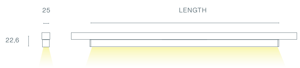
DIMENSIONS (mm)
