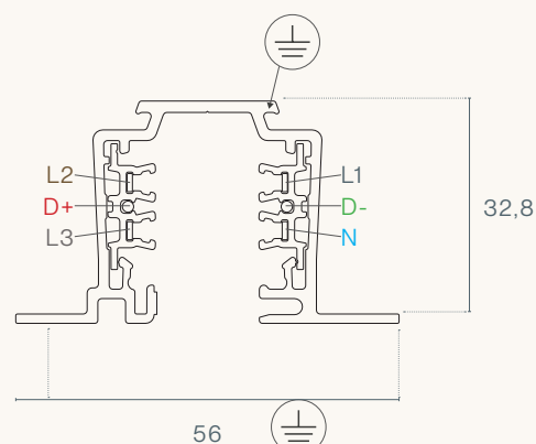
Dimensions (mm)
