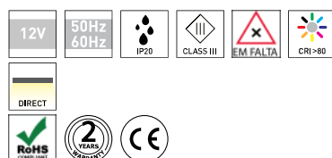
2002-116 ECO 14,4W 120LED PRODUCT TABLE AND TECHNICAL SPECIFICATIONS - ECO SMD2835 14,4W 120 LED IP20
