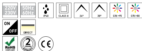
LORY 12W PRODUCT TABLE AND TECHNICAL SPECIFICATIONS - CRI→80
