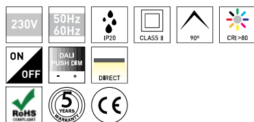
MATRIX EVO 1200X300MM PRODUCT TABLE AND TECHNICAL SPECIFICATIONS - CRI>80
