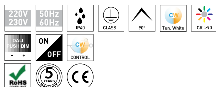
ORIS NEO D/I LS SUSP. OP. PRODUCT TABLE AND TECHNICAL SPECIFICATIONS - CRI>90
