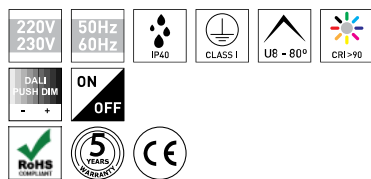
ORIS SL. PRO C. D/I PR+LG PRODUCT TABLE AND TECHNICAL SPECIFICATIONS - CRI→90
