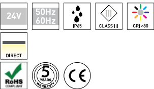
2002-126 14,4W 60LED PRODUCT TABLE AND TECHNICAL SPECIFICATIONS - EFFICIENCY SMD5050 14,4W 60 LED IP65
