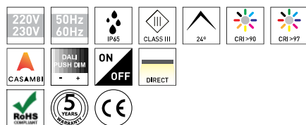
TYR 11W - IP65 PRODUCT TABLE AND TECHNICAL SPECIFICATIONS - CRI→90
